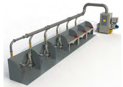
examples of installation with a central collector.
